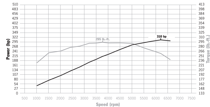
Panamera and Panamera 4: 310 horsepower at 6200 rpm, 295 lb.-ft. at 3750 rpm
